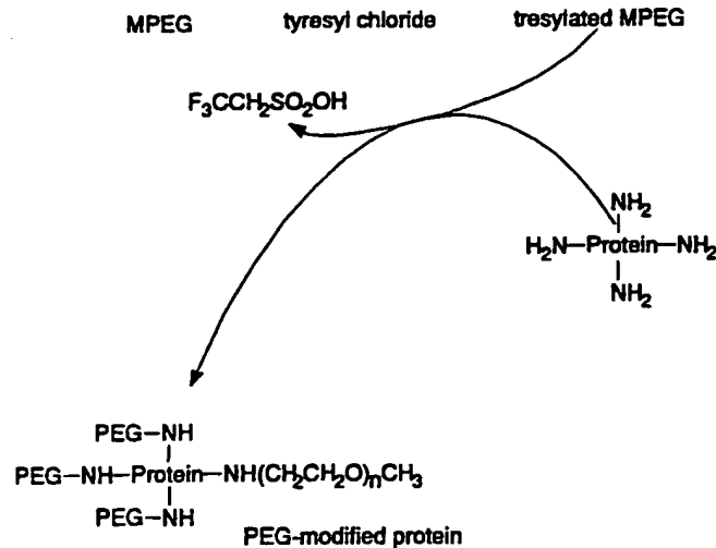
Scheme 1. Reactions involved in the activation of MPEG with tresyl chloride and the subsequent coupling of the activated polymer to amino groups in a protein (from Delgado et al., Id.).
